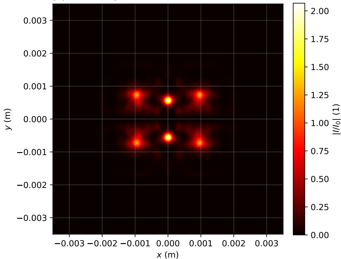
Intensity profile I(x, y, z = 1.274)/I_0 , P_{in}=9.0P_{cr} , artificial time
